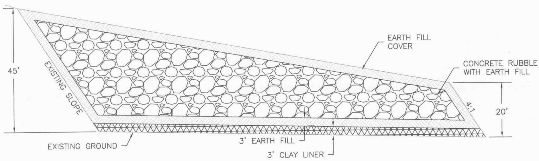
TYPICAL CROSS SECTION A-A' NTS
