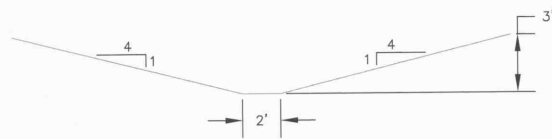
TYPICAL DITCH CROSS SECTION NTS
