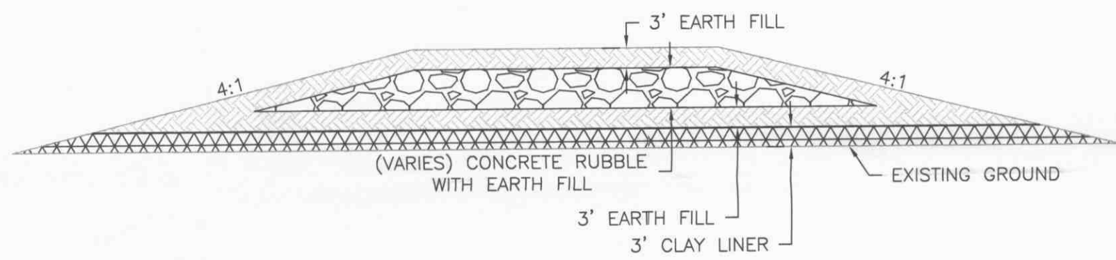
TYPICAL CROSS SECTION B-B' NTS
